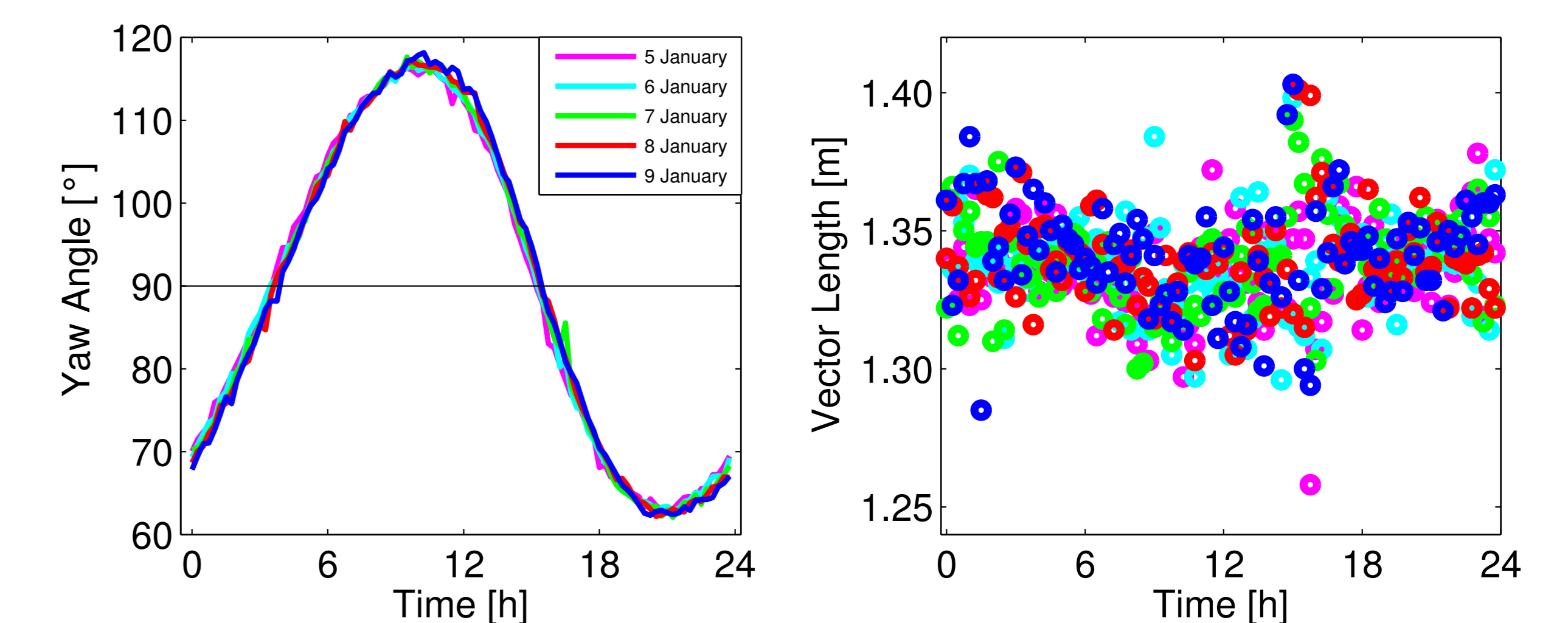
FIGURE 6: Estimated yaw angle (left) and vector length (right) for 5 days in January 2011.
